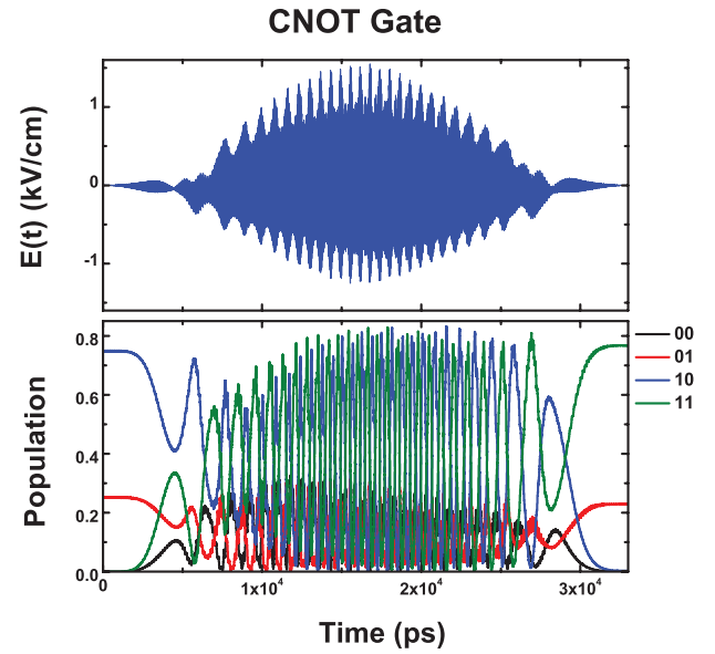
FIG. 5. Optimized laser pulse for realizing the CNOT gate. The initial and target states are listed in Table III. In the lower panel, the population evolution is driven by the CNOT pulse. The initial state is \cos(\frac{\pi}{3})|01\rangle + \sin(\frac{\pi}{3})|10\rangle . After population oscillations due to the effect of the laser pulse, the final qubit populations are 0.00363 ( |00\rangle ), 0.25807 ( |01\rangle ), 0.00273 ( |10\rangle ), and 0.73546 ( |11\rangle ). The populations of state |10\rangle and |11\rangle are switched, which confirms the correctness of the converged laser pulse.
